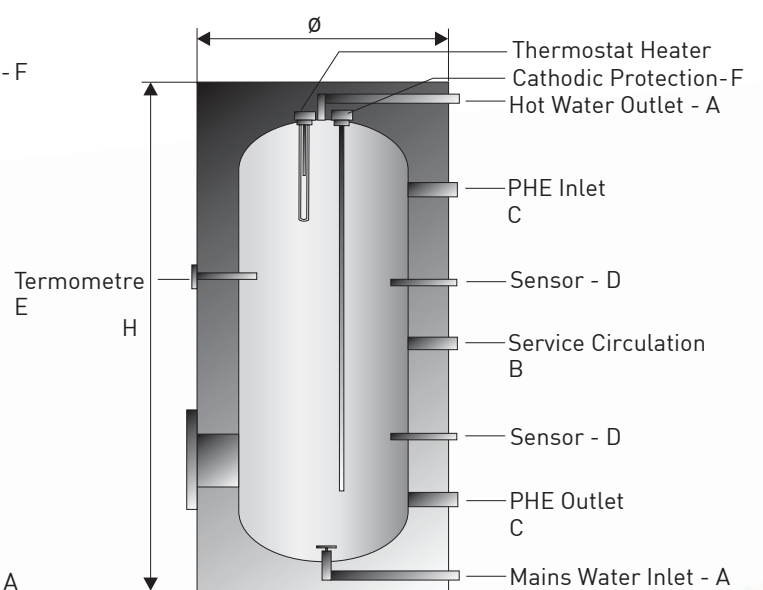
Accumulator Tank
