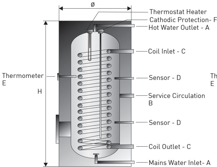
Single Serpentine Boiler
